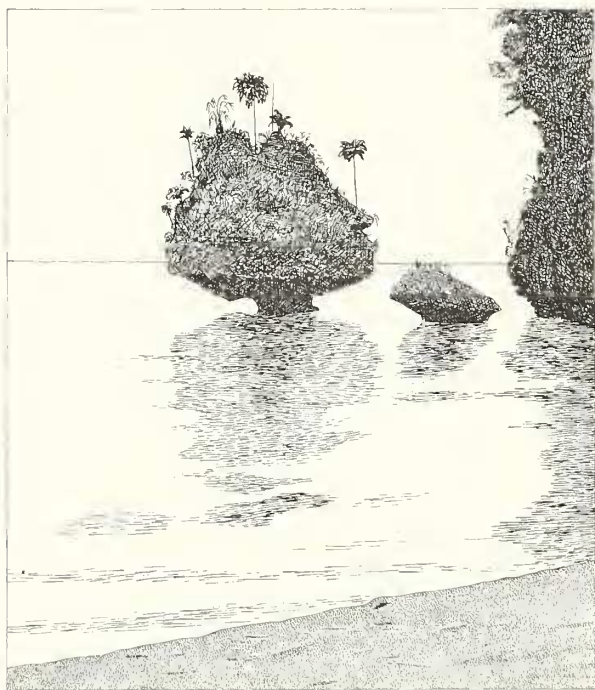
TEXT-FIG. 1. A 'toadstool island' from the north coast of Batoe Daka, Togian Islands, Celebes, sketched after Umbgrove (1939, fig. 21). The intertidal notch is chiefly eroded by Echinometra mathaei .
